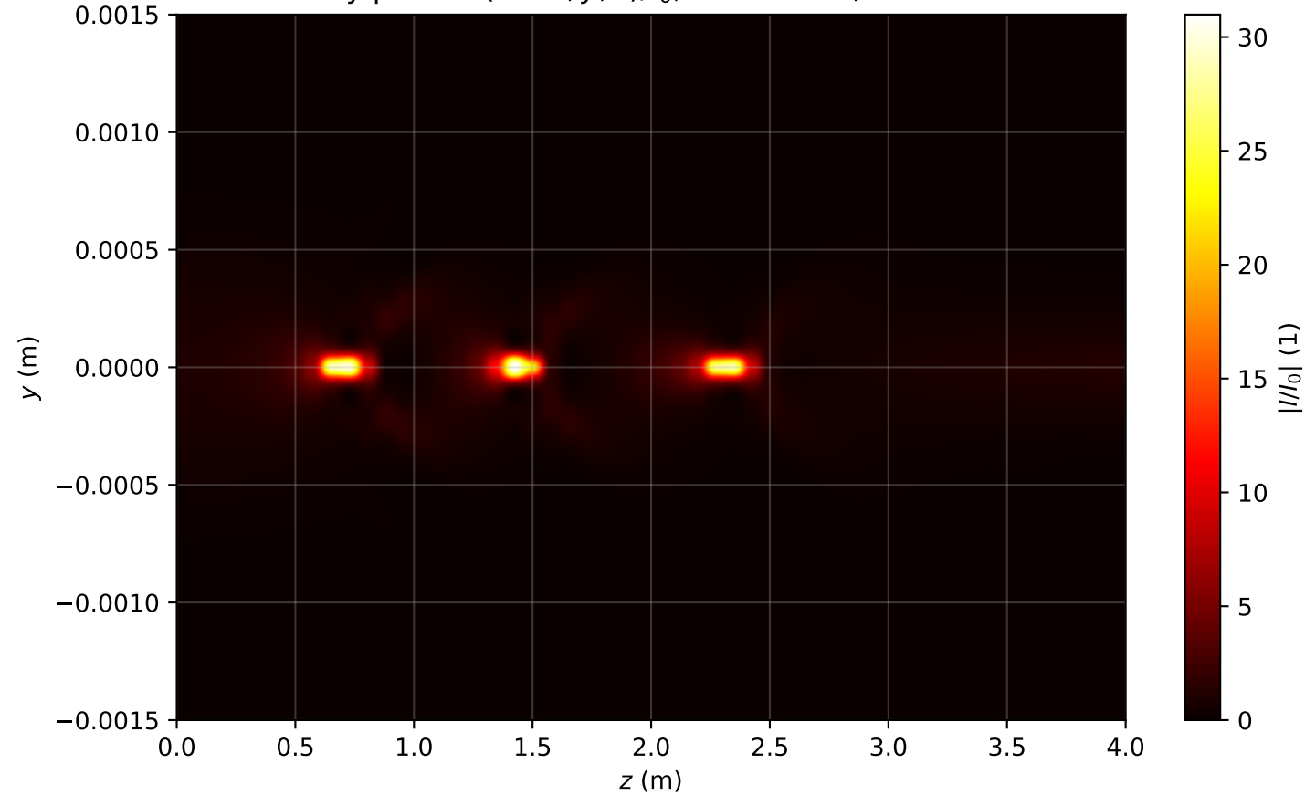
Intensity profile I(x=0, y, z)/I_0 , P_{in}=3.5P_{cr} , artificial time
